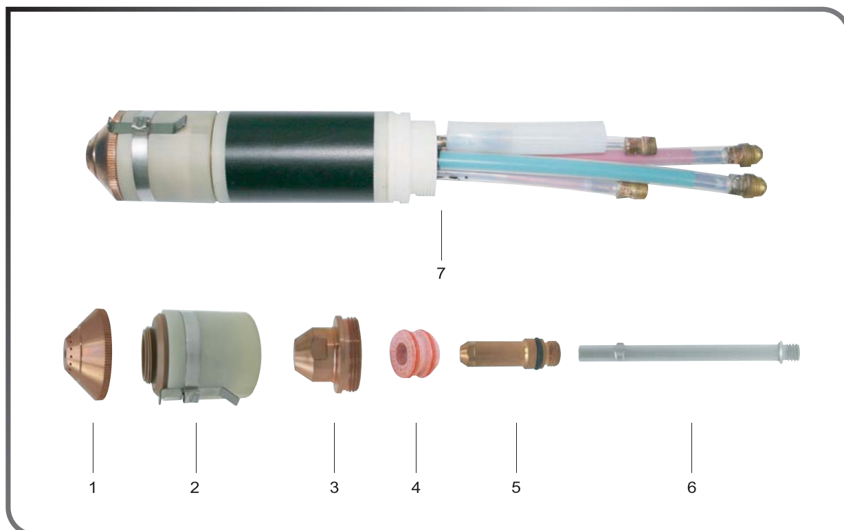
TW-MAX200 HYPERTHERM MAX200
